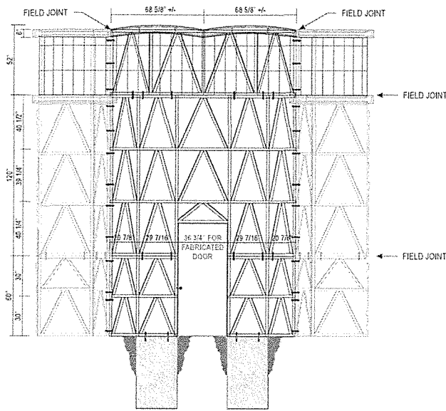
BACK VIEW
